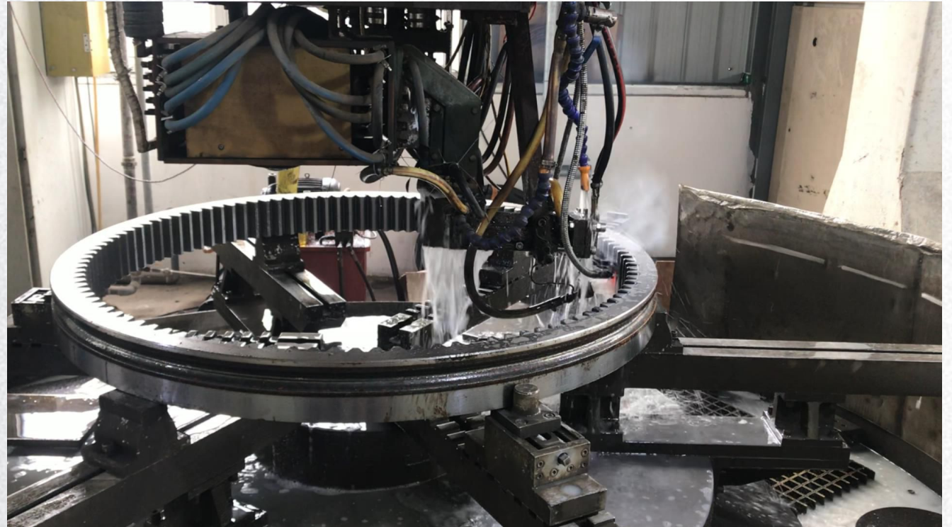
Quenching equipment
